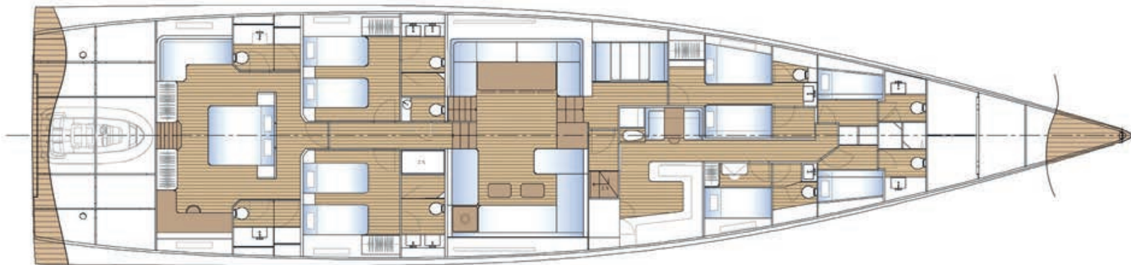
INTERIOR PLAN
